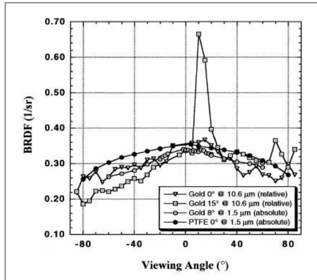
Figure 78. Hanssen's published IR BRDF measurements of Spectralon® and Infragold® [29].
